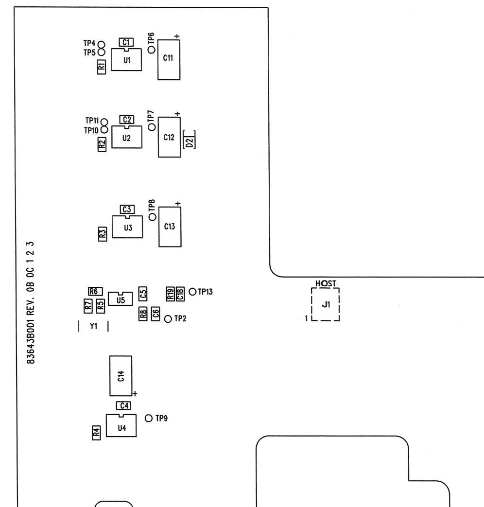
SOLDER SIDE
