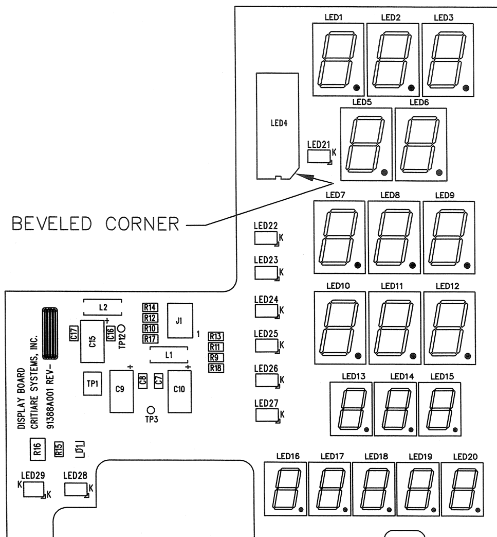
COMPONENT SIDE
