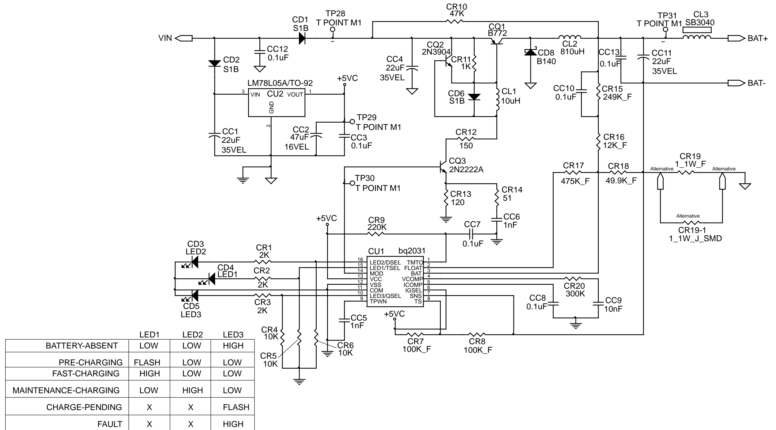
Figure 47: Battery Charger Schematic Diagram
