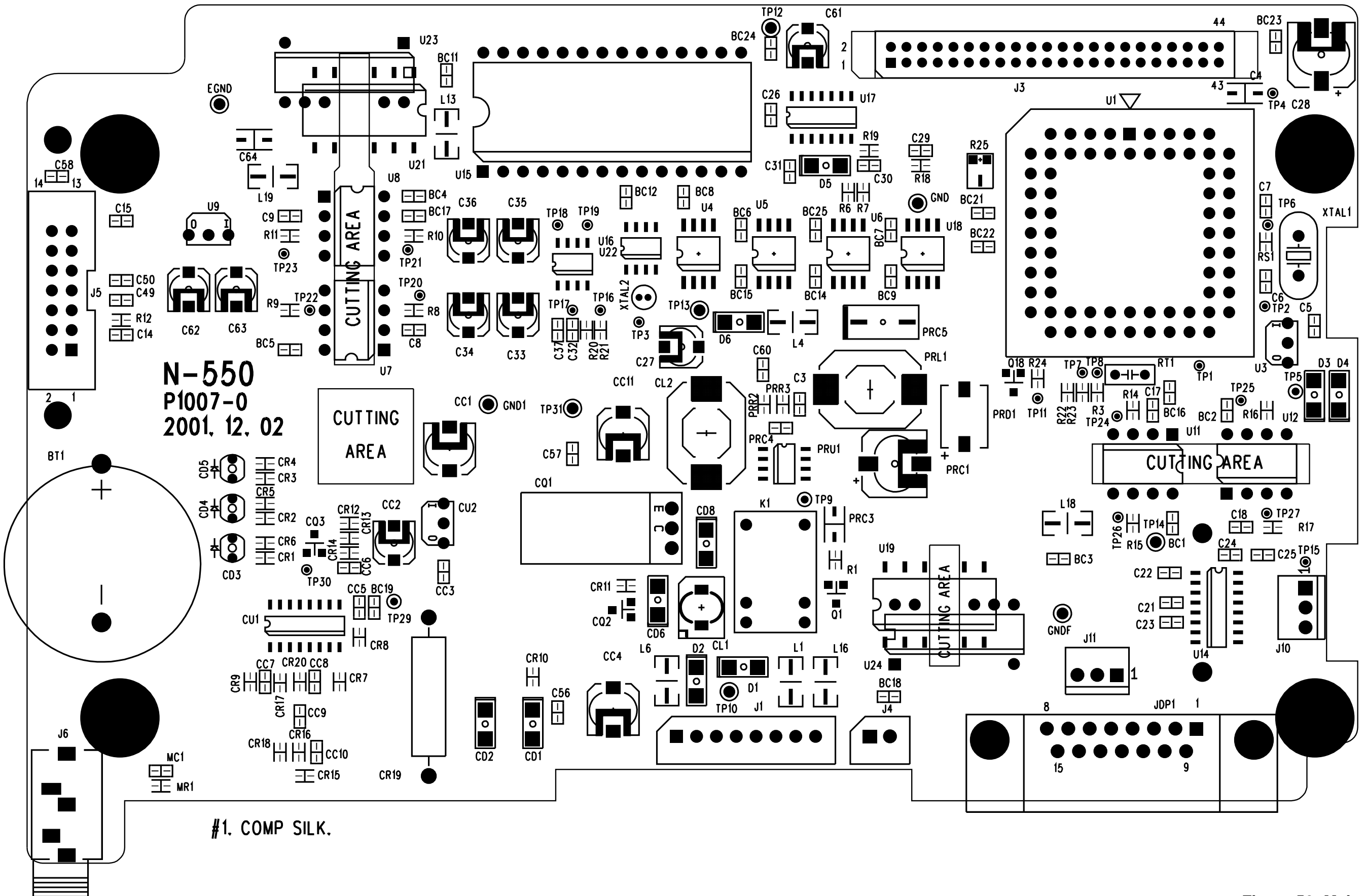
Figure 56: Main PCB Parts Locator Diagram
