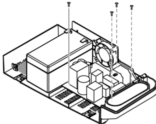
Figure 29: Power Supply Screws
